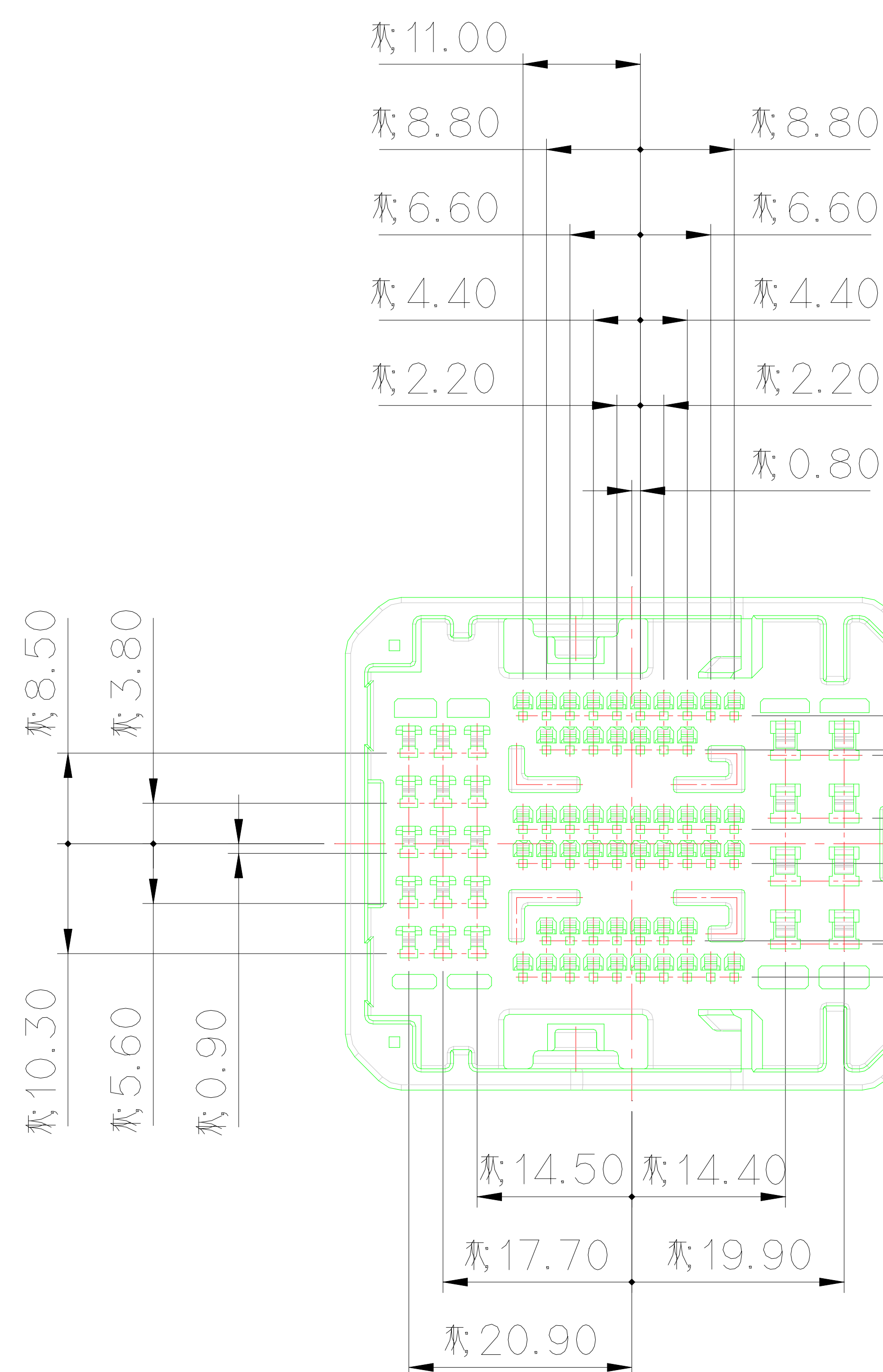
PITCH DETAIL
