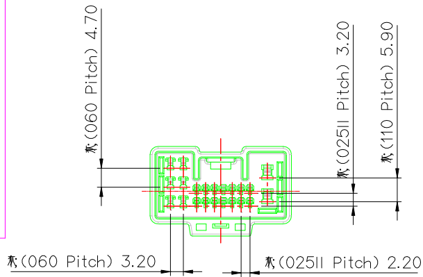
PITCH DETAIL
