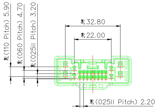
PITCH DETAIL
