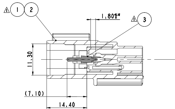
SECTION A-A (025)
