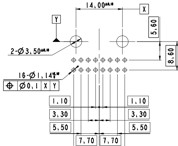
RECOMMENDED PCB LAYOUT (GENERAL TOLERANCE : \pm 0.1 ) (MOBIS WAVELESS 공법 전용)
