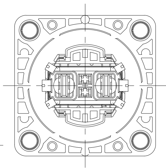
BACK VIEW (S=2/1)
