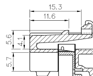
SECT. A-A
