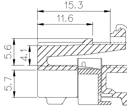
SECT. A-A
