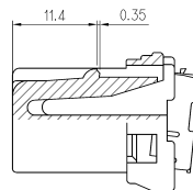
SECT. A-A
