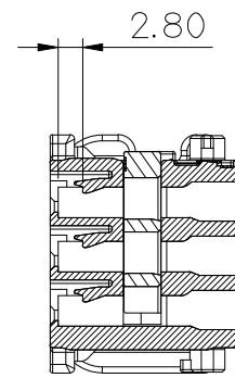
SECTION B-B (187)
