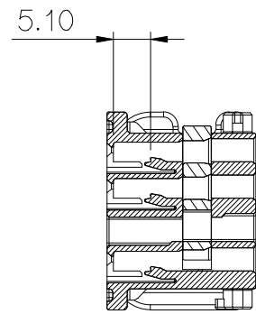
SECTION A-A (090)
