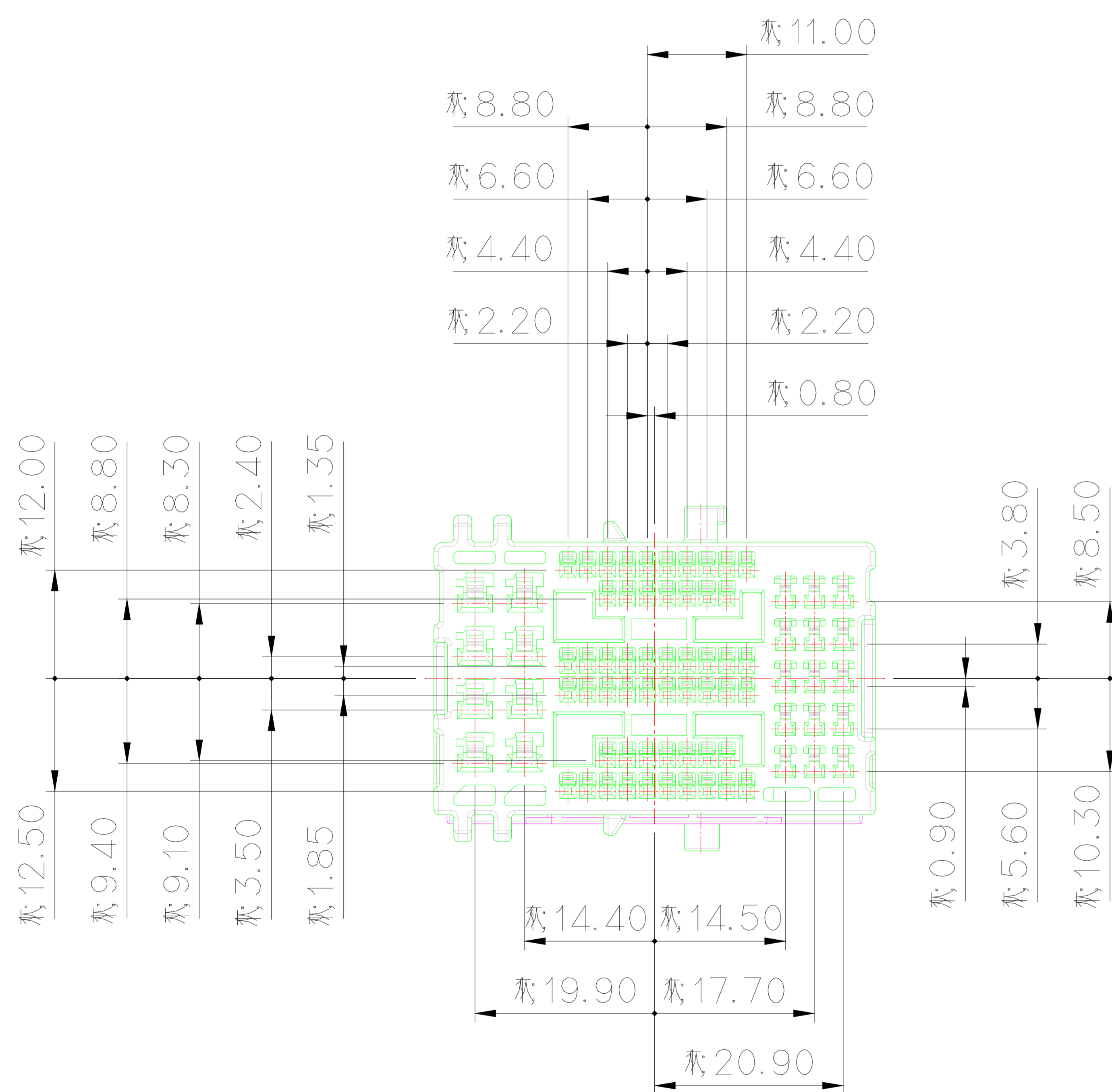
PITCH DETAIL
