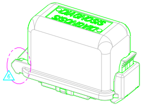
HOUSING/COVER 조립상태
