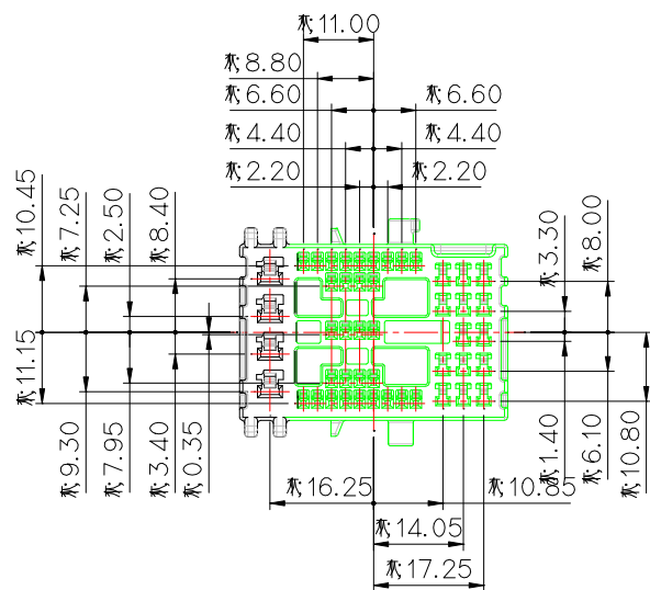
PITCH DETAIL
