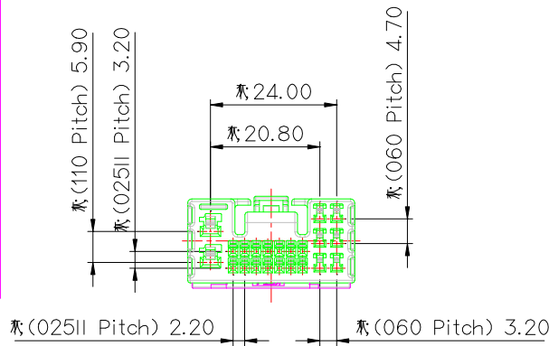
PITCH DETAIL
