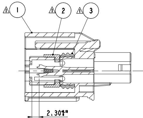
SECTION A-A(025)
