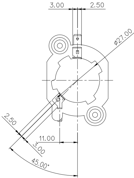
TERMINAL POSITION
