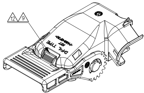
ISO VIEW (S= 1/2)
