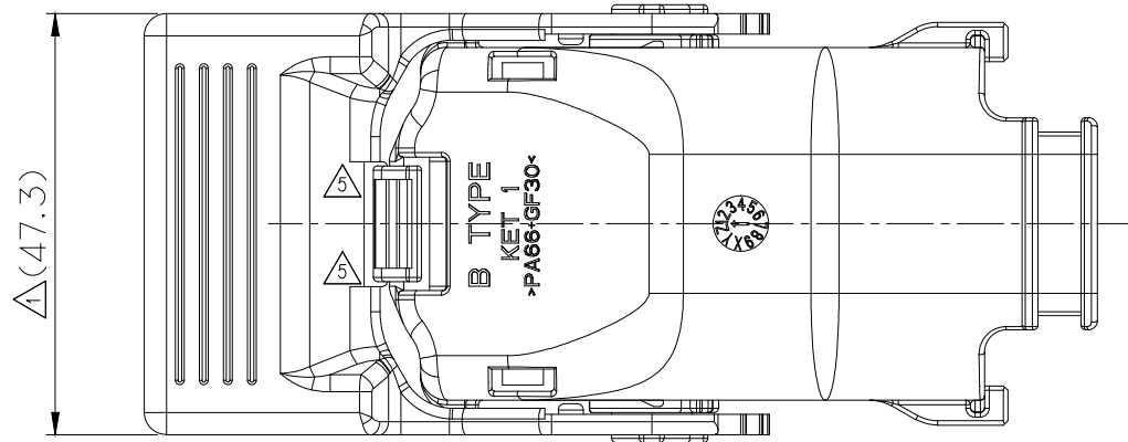
< LEVER OPEN >
