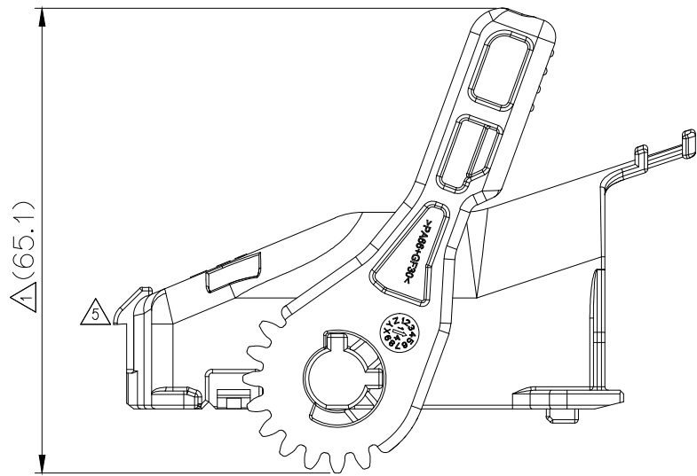
< LEVER OPEN >
