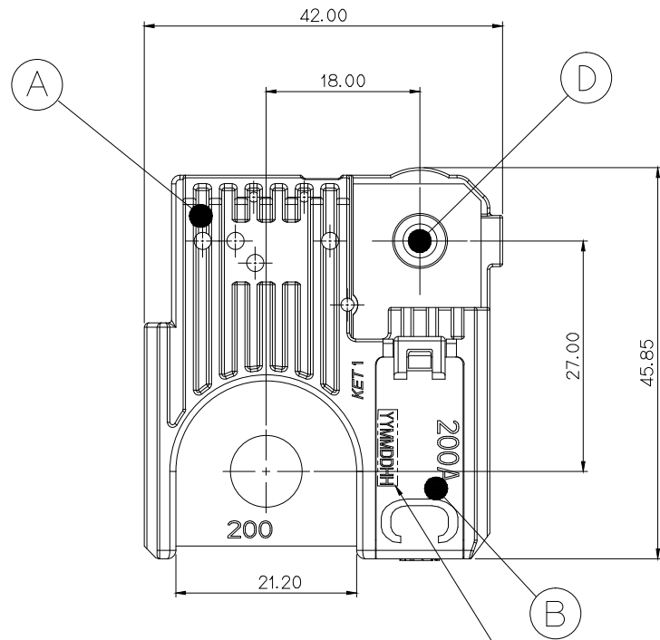
DETAIL "Z" (LOT No.)
