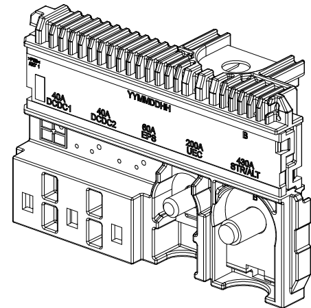
ISO VIEW
