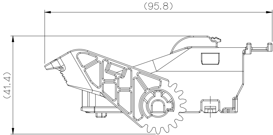
< LEVER OPEN >
