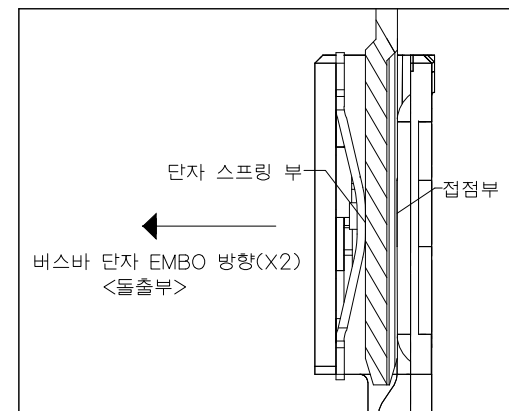
DETAIL "C" (S= 5/1)
