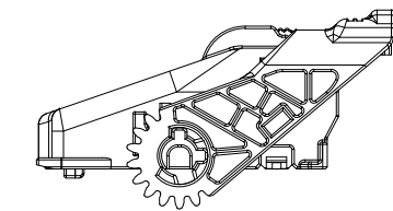
DELIVERY CONDITION ( CLOSED LEVER )
