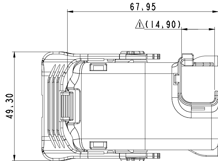
LEVER OPEN
