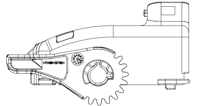
DELIVERY CONDITION CLOSED LEVER
