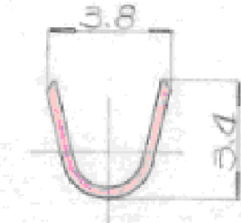
SECTION B-B (5/1)
