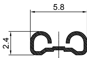
SECTION A-A (5/1)
