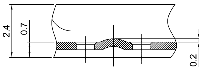
DETAIL 'D' (10/1)
