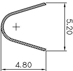
SECTION 'C-C' (SCALE 5/1)
