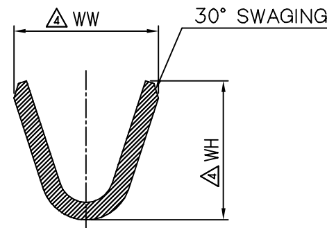
SECTION B-B (S:10/1)
