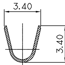
SECTION A-A' (SCALE 5/1)
