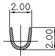
SECTION B-B' (SCALE 5/1)
