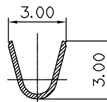
SECTION B-B' (SCALE 5/1)
