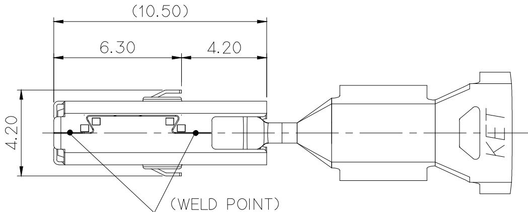
N110 WP FEMALE TML (SCALE 1:1)
