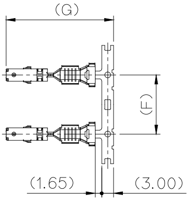
N110 WP FEMALE TML (SCALE 1:1)
