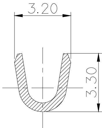
SECTION A-A' (5/1)
