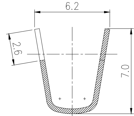
SEC. B-B (S=1/5)
