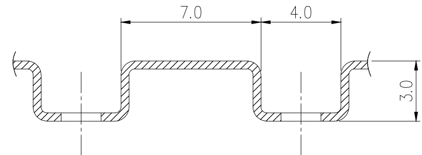
SEC. C-C (S=1/5)
