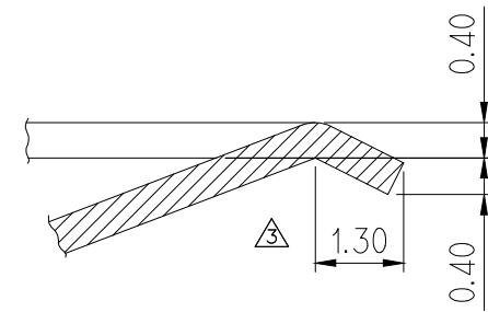
DETAIL "D"(S=1/10)
