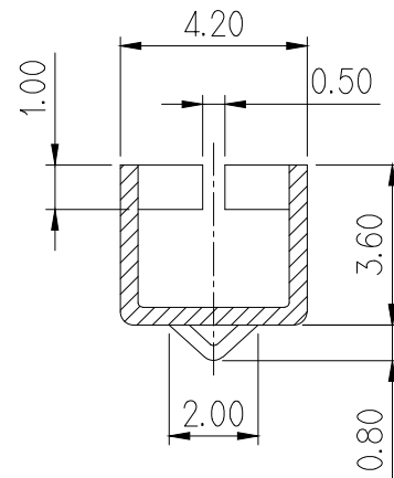
SECTION C-C
